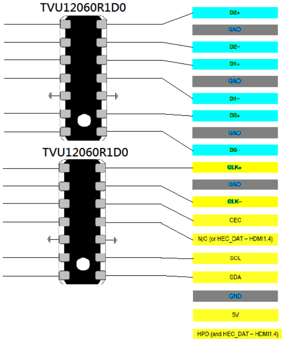
HDMI block Diagram
